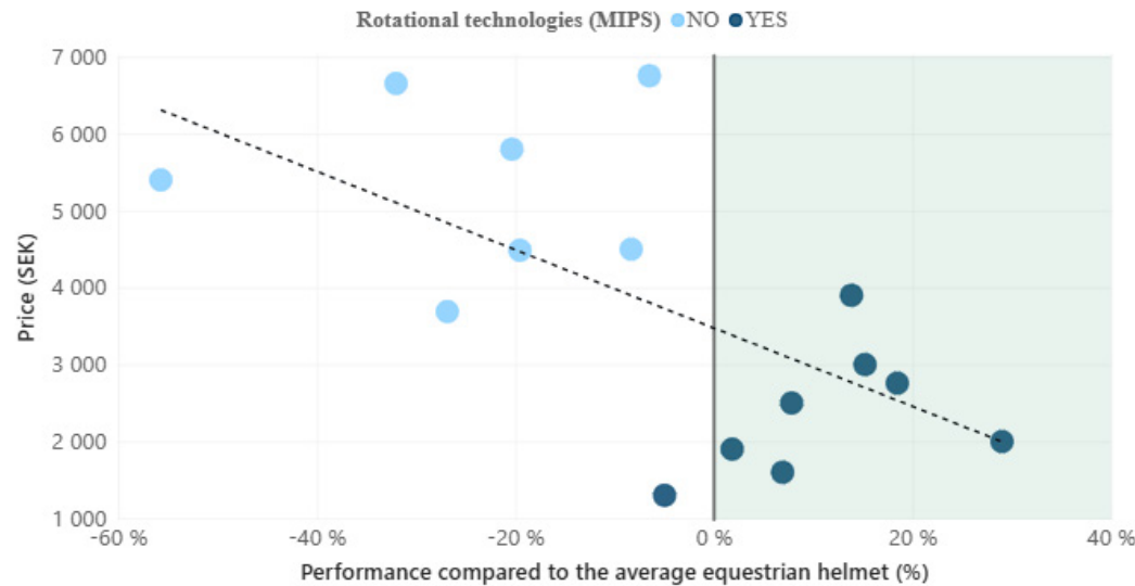
Figure 1. Test performance compared with price for helmets with and without rotational technologies (Mips).
