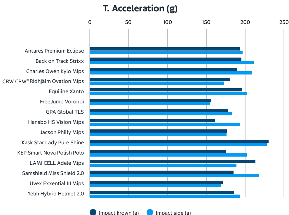
Figure 2. Shock absorption measuring linear acceleration
